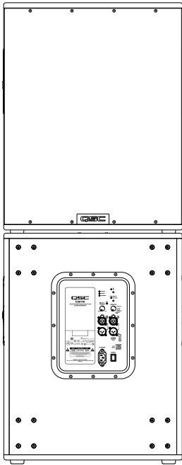
CS18 double stacked in cardioid deployment
